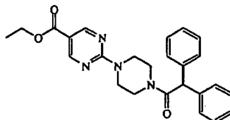
intermediate 5
